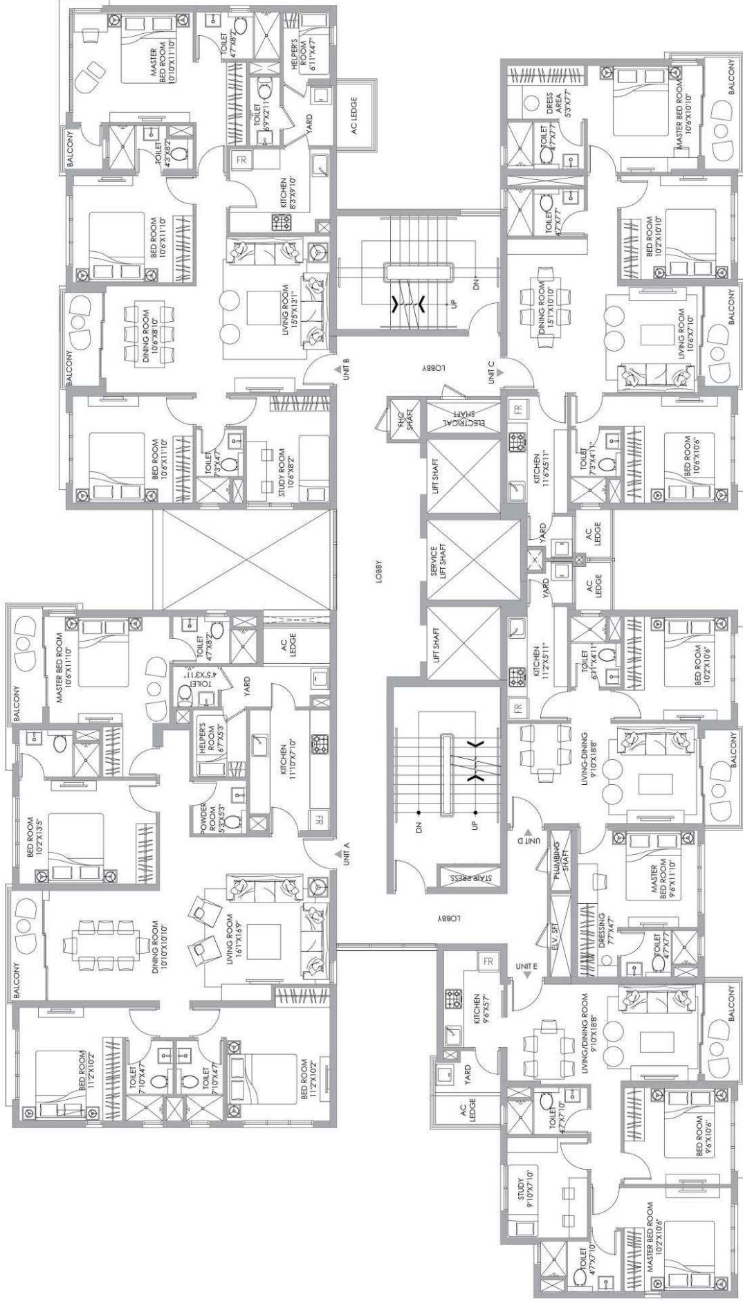
TYPICAL FLOOR PLAN: BLOCK 9
