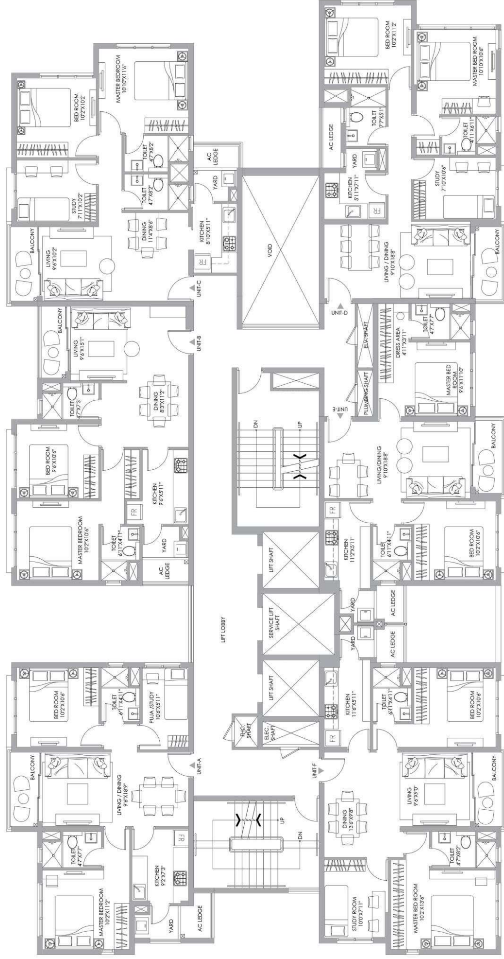
TYPICAL FLOOR PLAN: BLOCK 8
